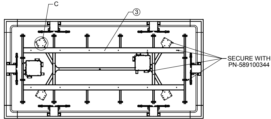
TOP VIEW: WKSF TOP/SPACER/SUBTOP REMOVED IN THIS VIEW
