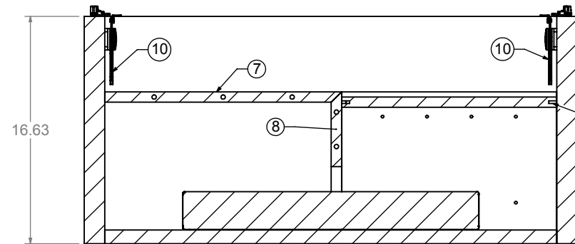
SECTION B-B
